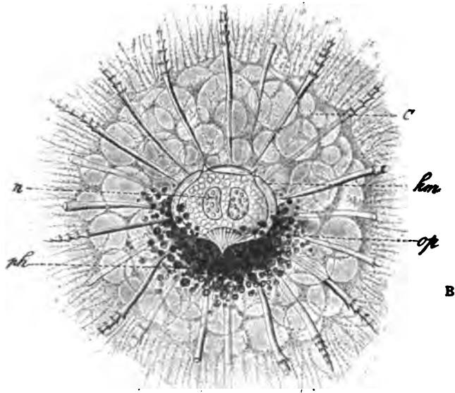
FIG. 26.—A, Lithocercus annularis , with sagittal ring (from Parker and Haswell). B, Aulactinium actinastrum . C, calymma; cent. caps., kn, central capsule; Ext. caps. pr., Extracapsular, and Int. caps. pr., intracapsular protoplasm; n, nu, nucleus; op, operculum; ph, phaeodium; psd, pseudopodium; Skel., skeleton; z, Zooxanthella. (From Lang's Comparative Anatomy , after Haeckel.)
